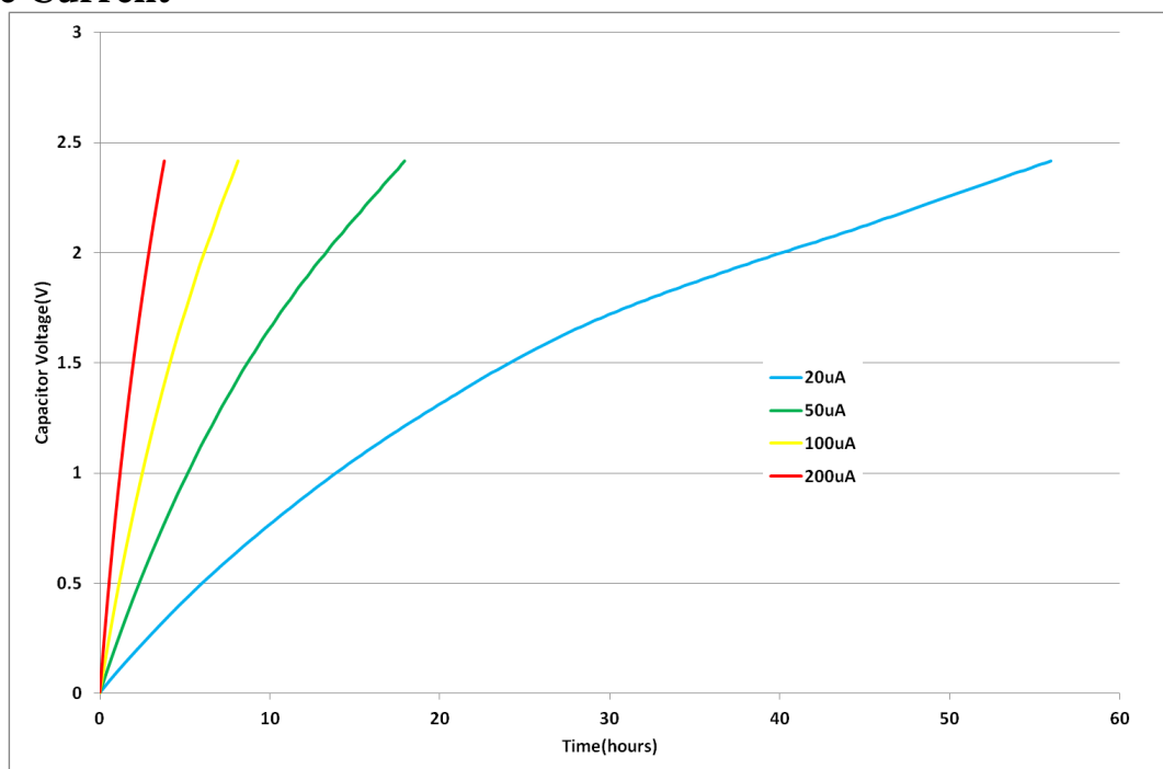
Fig 11: Charging an HW101 with low current
