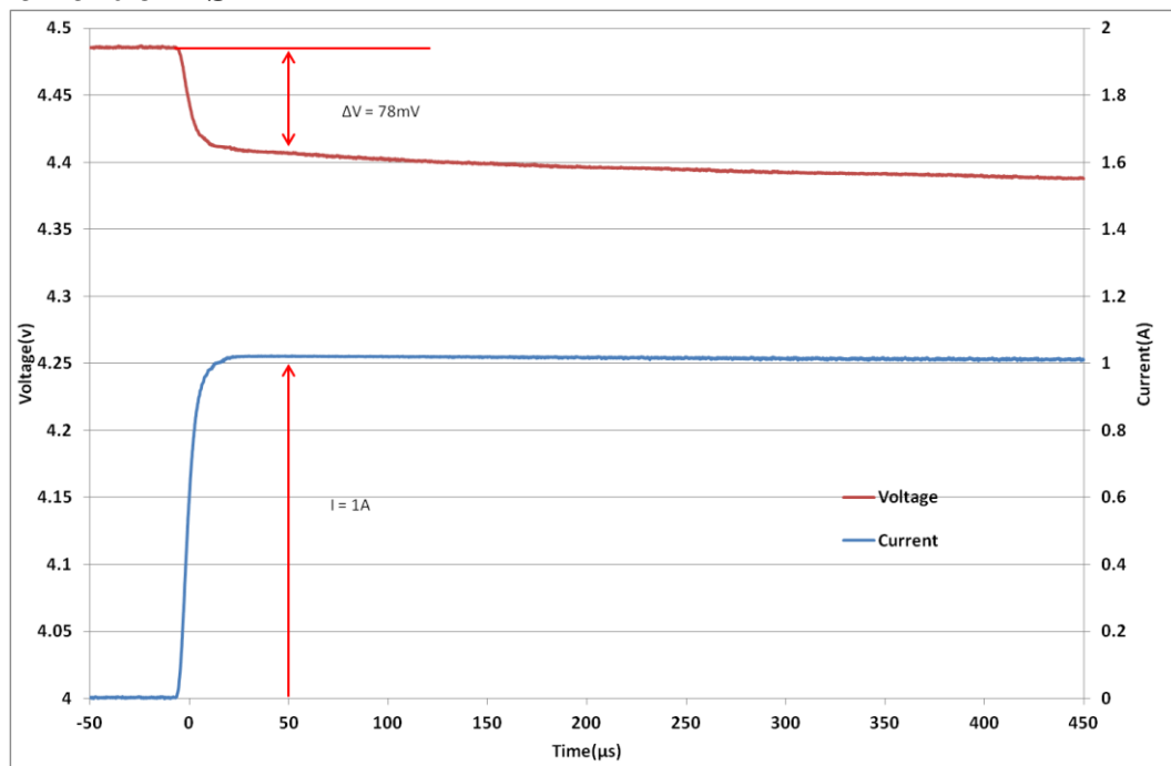
Fig 3: Measurement of ESR for a GZ215
