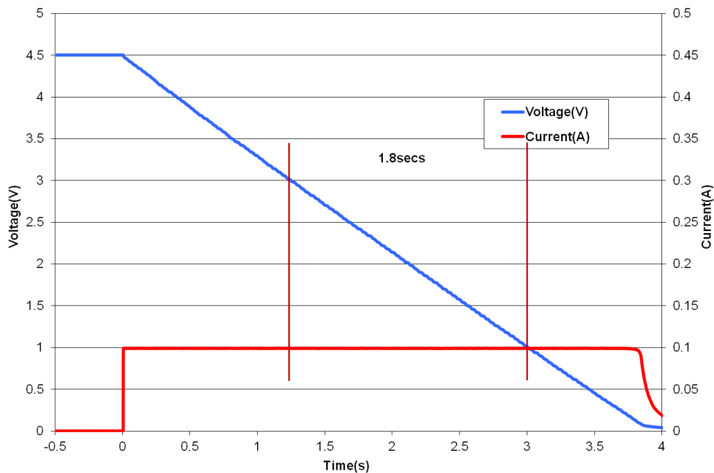
Fig 2: Measurement of DC Capacitance for a GZ215
