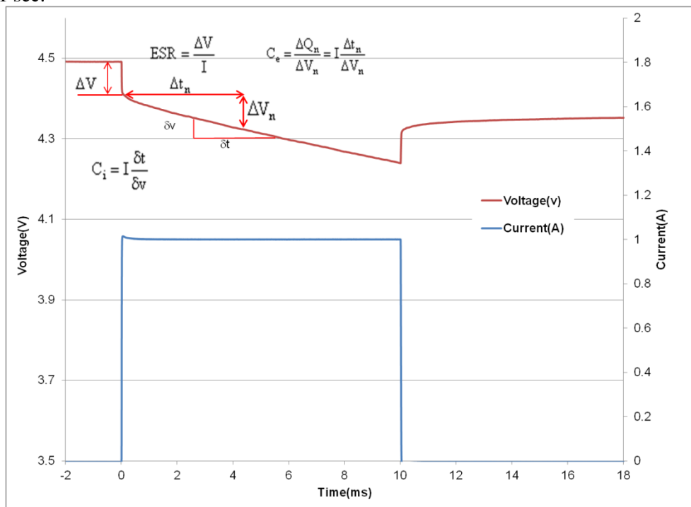
Figure 1: Effective capacitance, instantaneous capacitance and ESR for a GZ215
