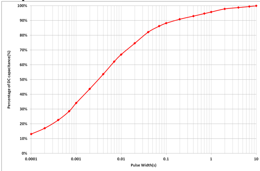
Figure 4: Effective Capacitance
