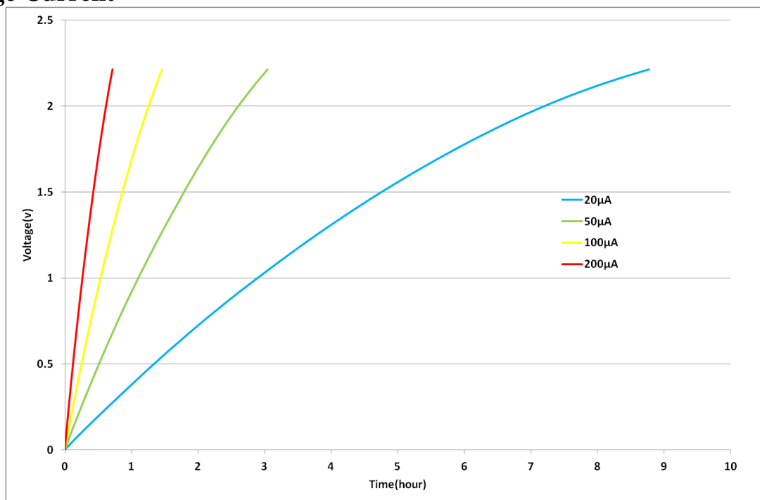
Fig 11: Charging a GZ115 with low current
