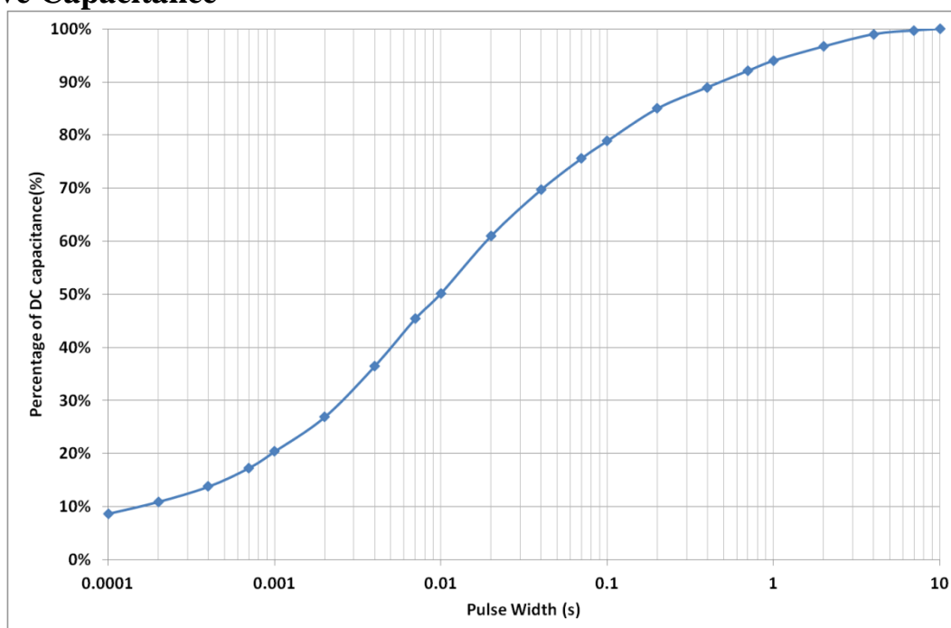
Figure 4: Effective Capacitance
