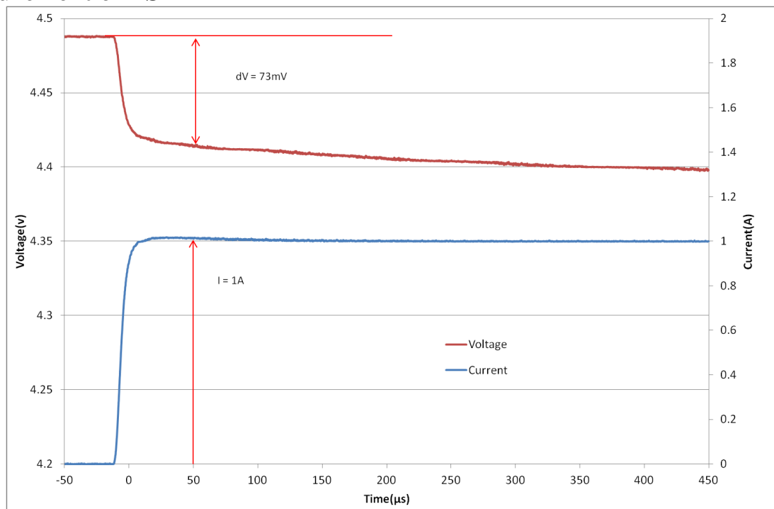
Fig 3: Measurement of ESR for a GA209
