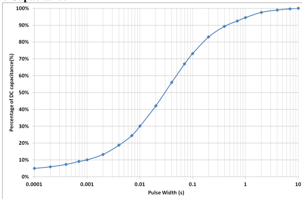
Figure 4: Effective Capacitance
