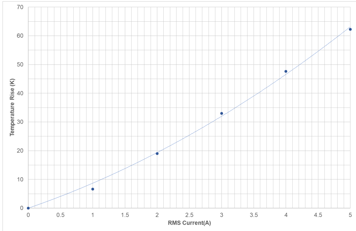
Fig 12: Temperature rise in DMT334R2S474M3DTA0 with RMS current
