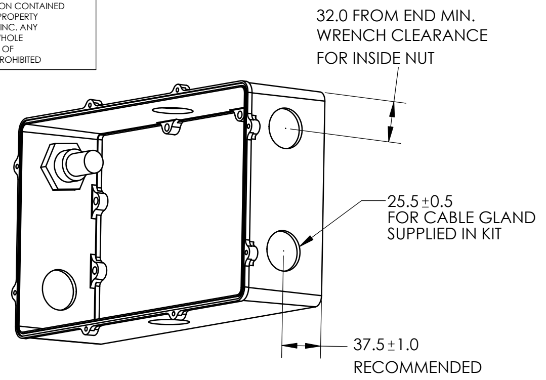
JUNCTION BOX DRILLING DIMENSIONS
