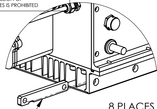
8 PLACES DETAIL G SCALE 1 : 3
