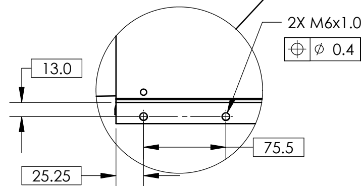
8 PLACES DETAIL D SCALE 2 : 7
