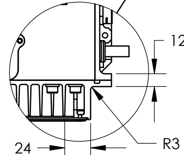
8 PLACES DETAIL J SCALE 2 : 7
